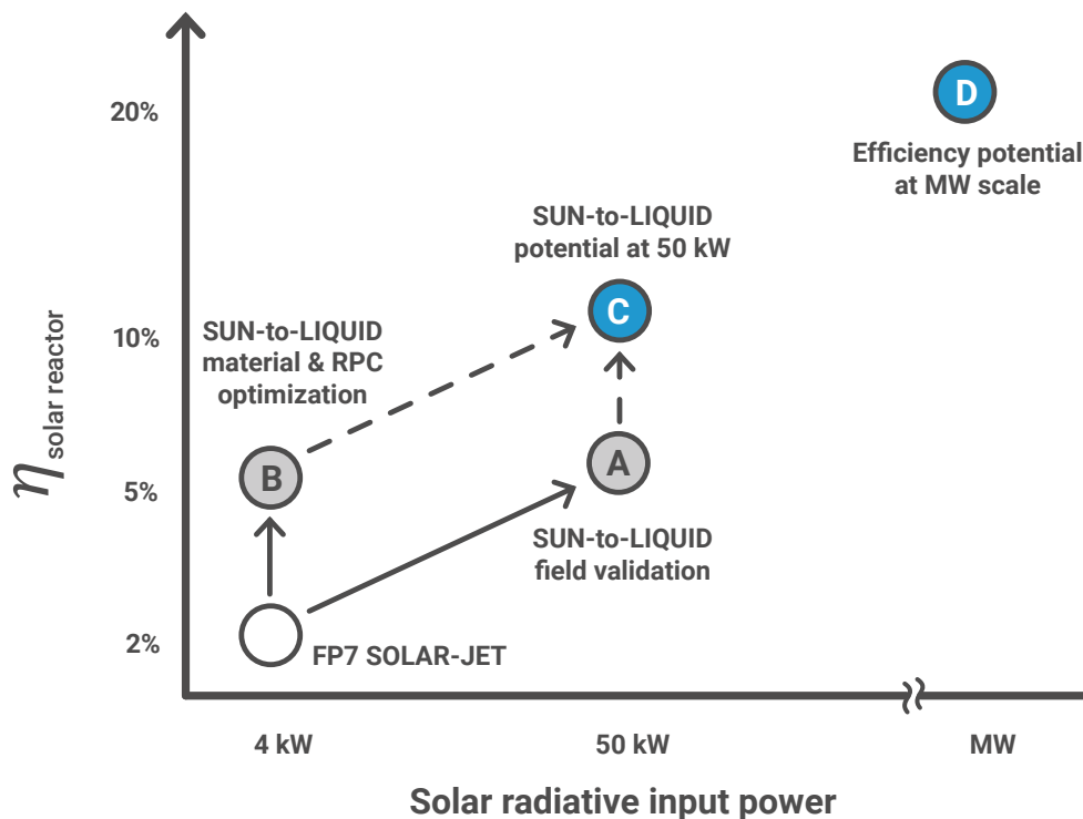
Figure 1: Roadmap towards competitive solar fuel production at large scale. The EU-FP7 project SOLAR-JET has achieved a solar reactor efficiency of 1.7% in a laboratory 4 kW setup. SUN-to-LIQUID aims at a solar reactor efficiency beyond 5%, enabled by scaling to a higher radiative power level (A) and material optimization (B). A combination of advanced materials
